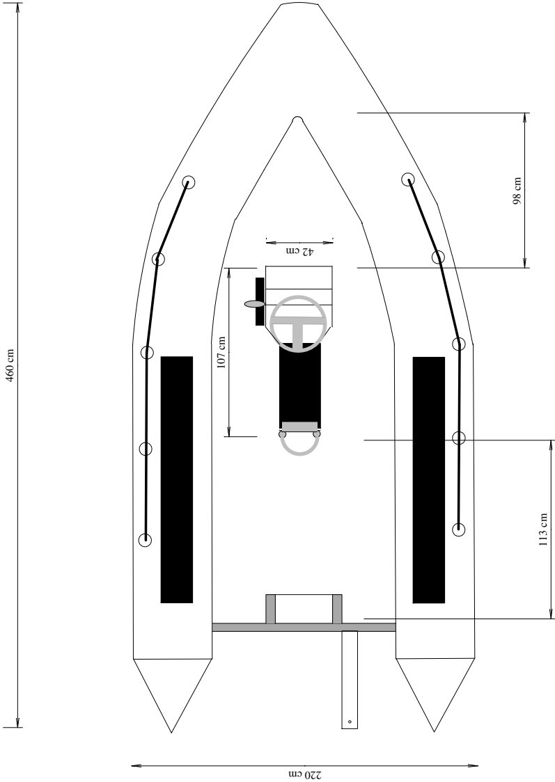
Double Module - Small Console
