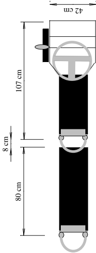
Double Module - Small Console
