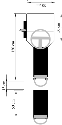
Single Module - Large Console
